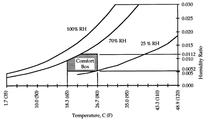
Figure 3.2-5 Human Comfort Levels to Temperature and Humidity
